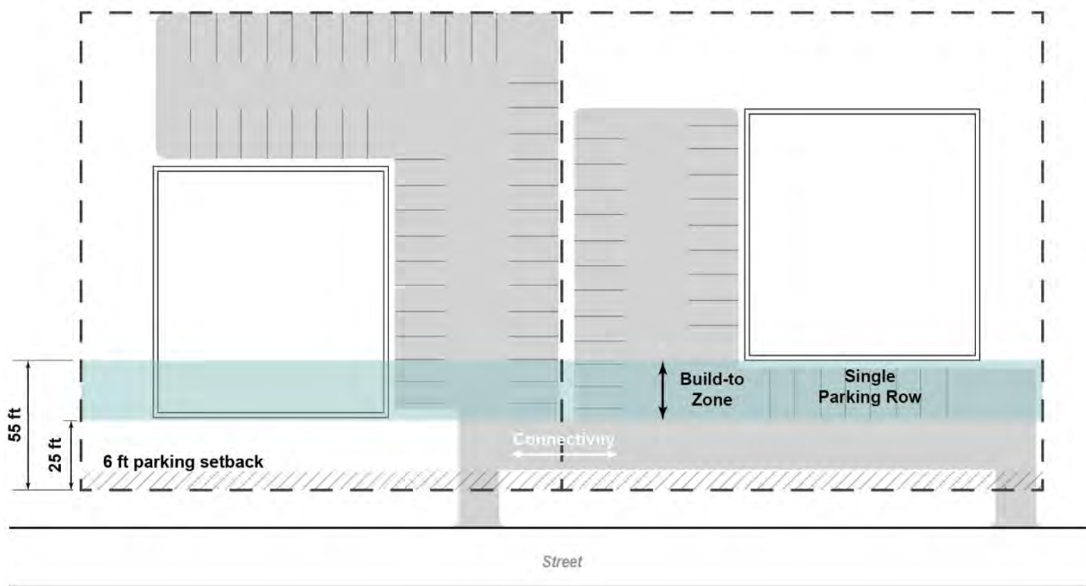
Figure 8-1 CCOD Build-To Zone, Parking Restriction, and Connectivity
