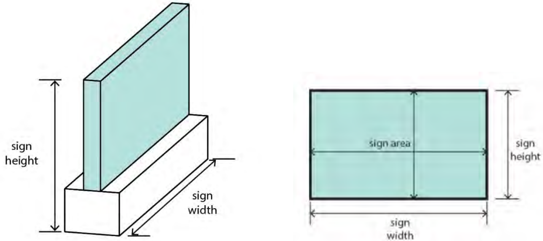
Figure 14-1 Sign Area and Height Measurement
