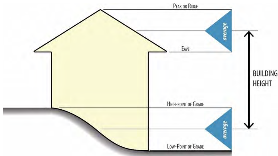
Figure 10-2 Building Height-Sloping Grade and Walkout
