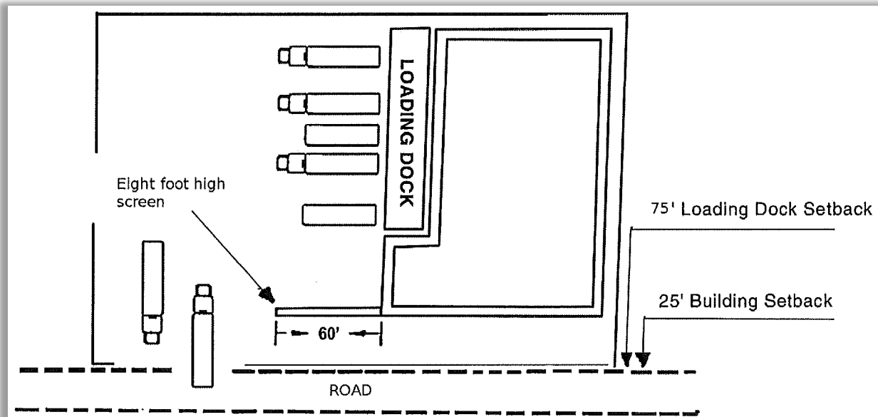
Figure 12-1 Loading Docks
