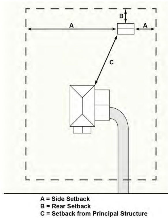
Figure 3-3 Spatial Requirements, Accessory Buildings
