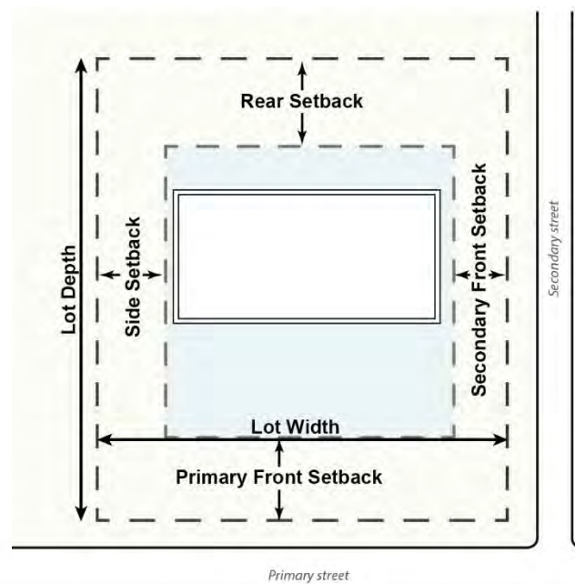
Figure 6-2 Spatial Requirements, Corner Lot
